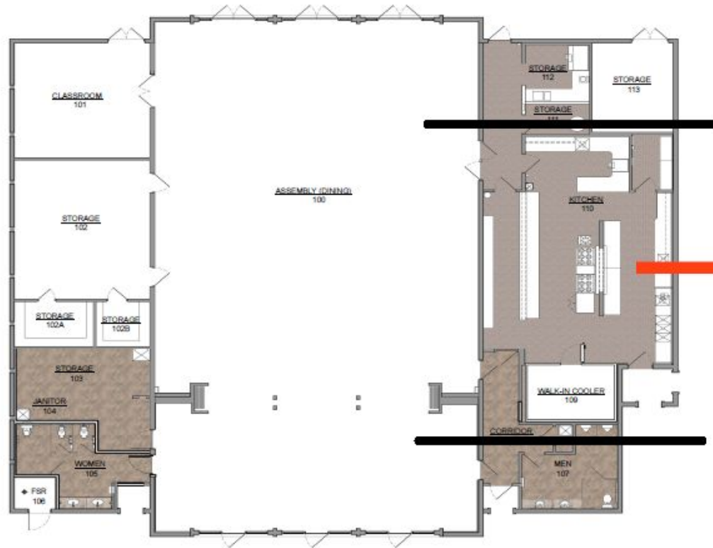
PRELIMINARY FLOOR PLAN SCALE: 1/8" = 1'-0"
